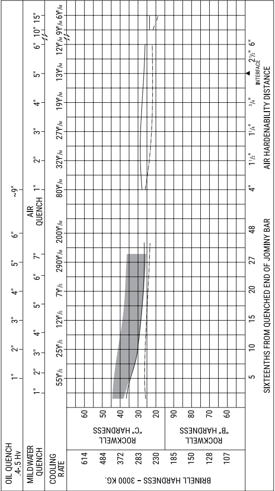
ROUND SECTION WITH SAME HARDNESS AT MID-RADIUS
